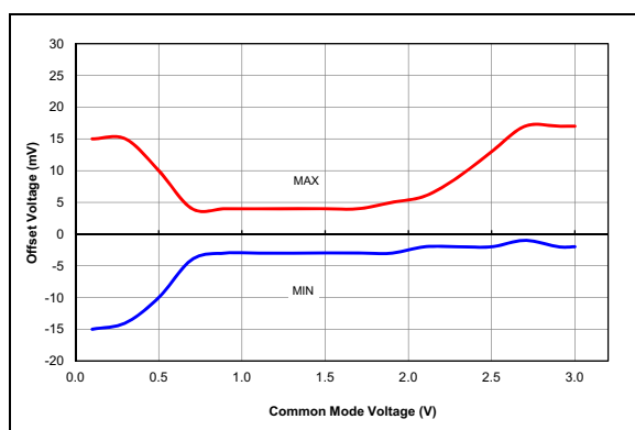
FIGURE 38-51: Comparator Offset, NP Mode ( CxSP = 1 ), V_{DD} = 3.0V , Typical Measured Values at 25^\circ C .
