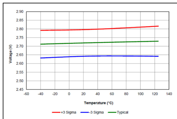
FIGURE 38-11: Brown-Out Reset Voltage, Trip Point (BORV = 00).
