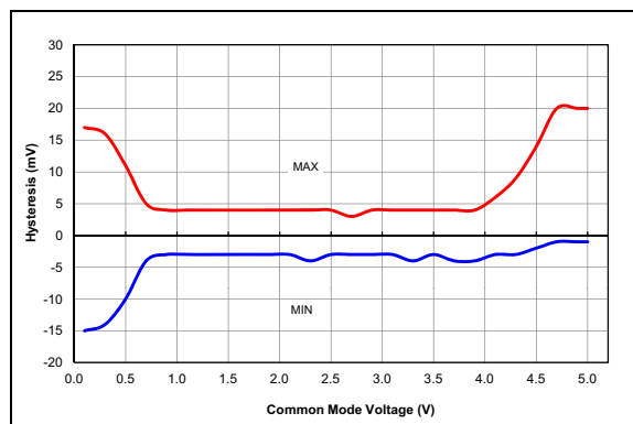
FIGURE 38-54: Comparator Offset, NP Mode ( CxSP = 1 ), V_{DD} = 5.0V , Typical Measured Values at 25^\circ C , PIC16F18856/76 Only.
