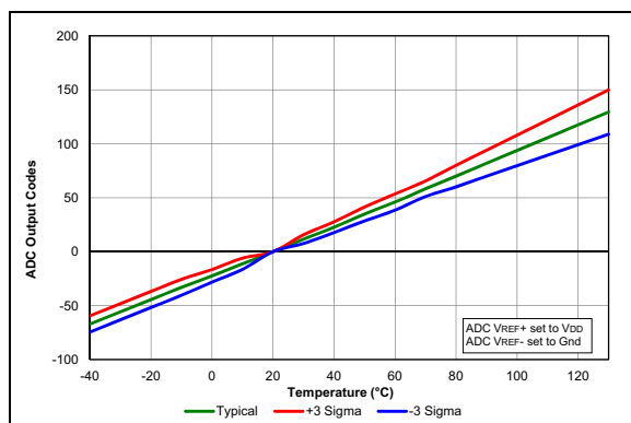
FIGURE 38-49: Temp. Indicator Slope Normalized to 20^\circ C , Low Range, V_{DD} = 2.3V .
