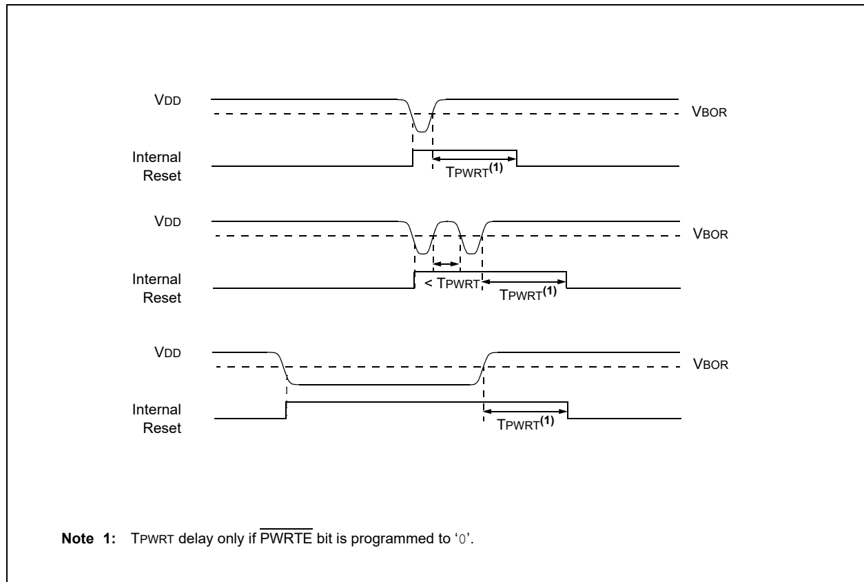
FIGURE 5-2: BROWN-OUT SITUATIONS
