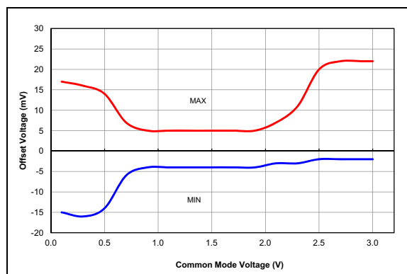
FIGURE 38-52: Comparator Offset, NP Mode ( CxSP = 1 ), V_{DD} = 3.0V , Typical Measured Values from -40^\circ C to 125^\circ C .
