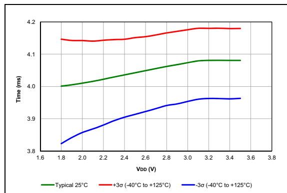
FIGURE 38-10: WDT Time-Out Period, PIC16LF18856/76 Only.
