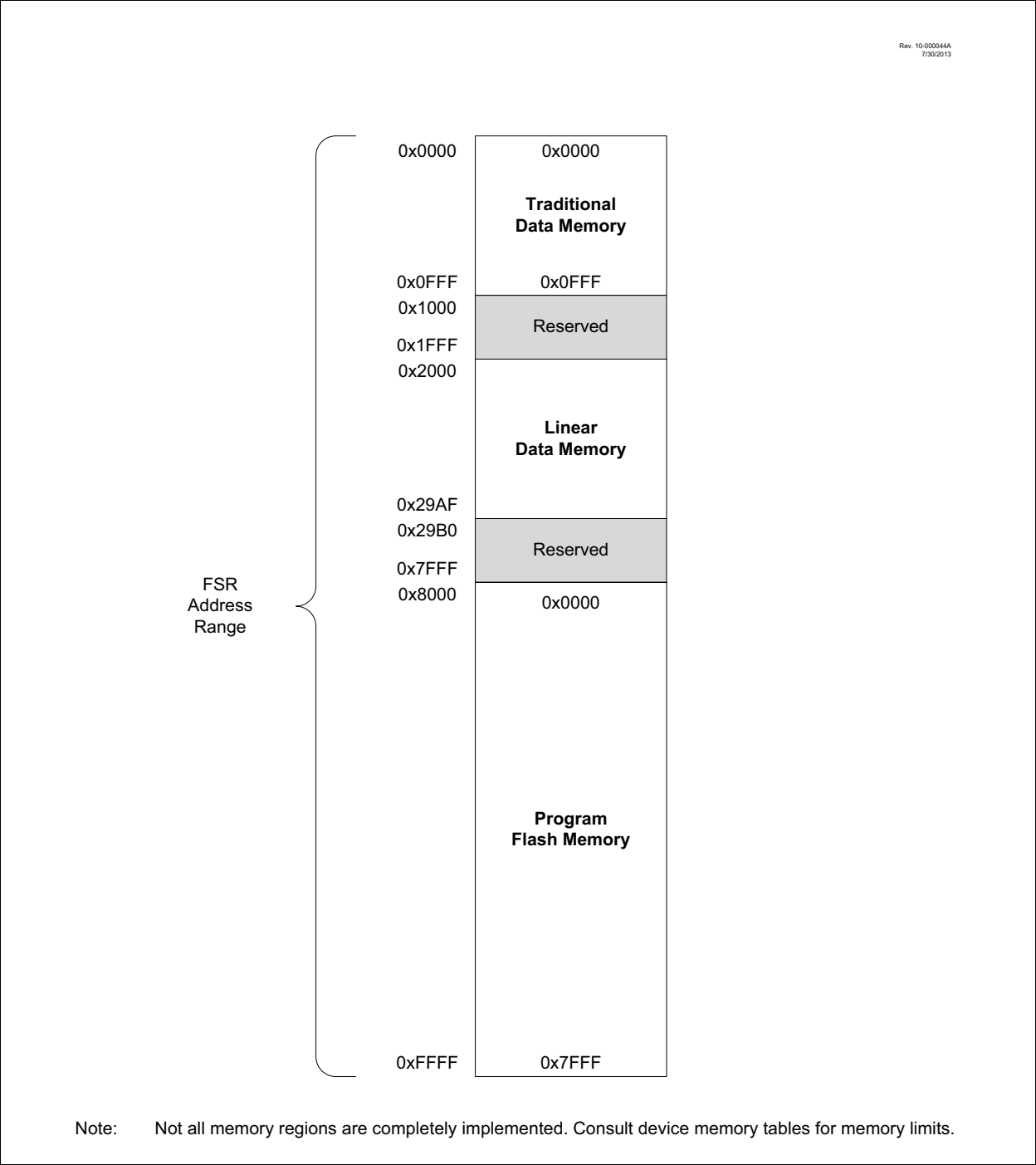
FIGURE 3-8: INDIRECT ADDRESSING
