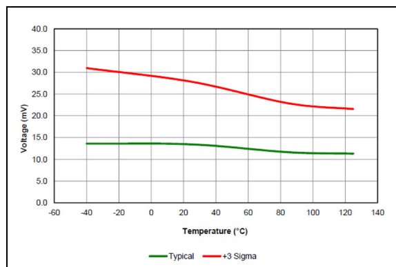
FIGURE 38-12: Brown-Out Reset Hysteresis, Low Trip Point (BORV = 00).
