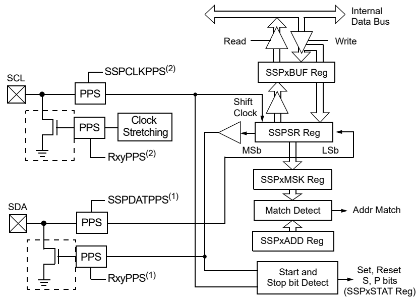
FIGURE 31-3: MSSP BLOCK DIAGRAM (I 2 C CLIENT MODE)
