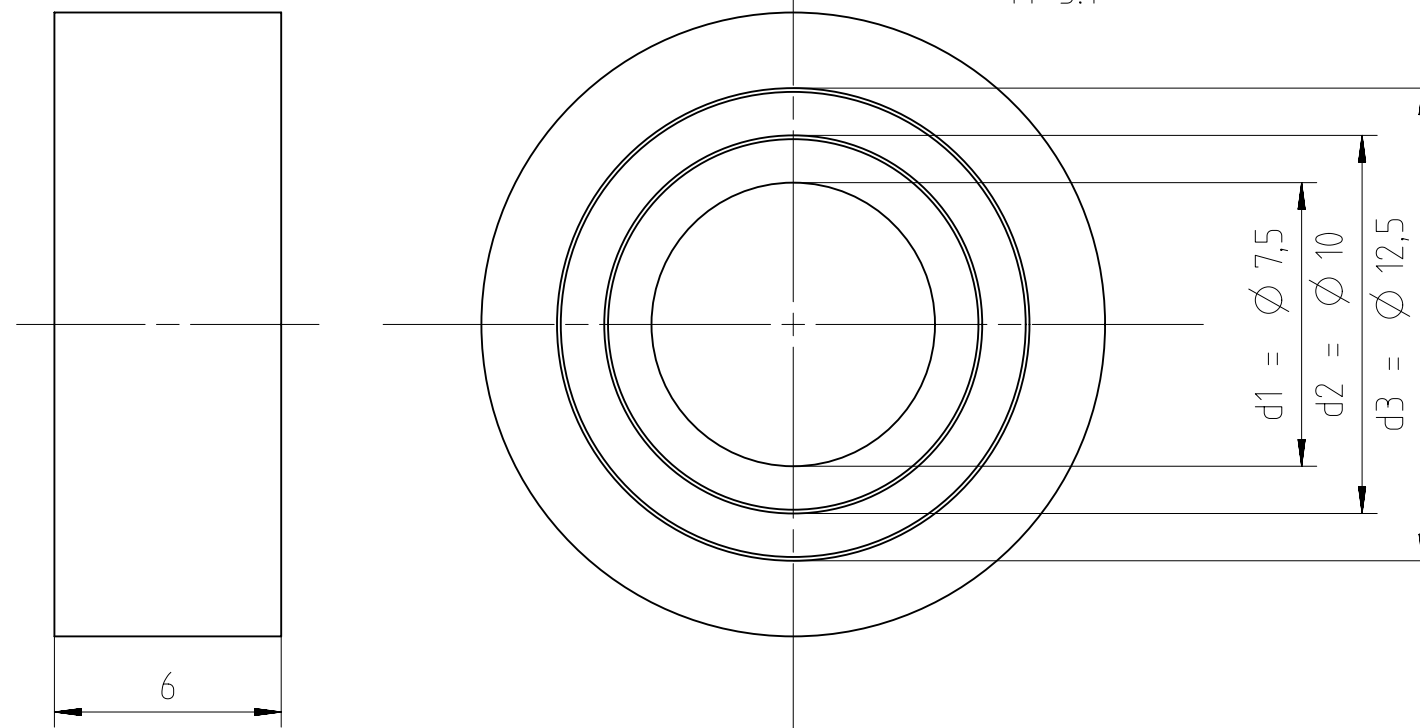
3 - Dichtring, ausschneidbar sealing with variable diameter
