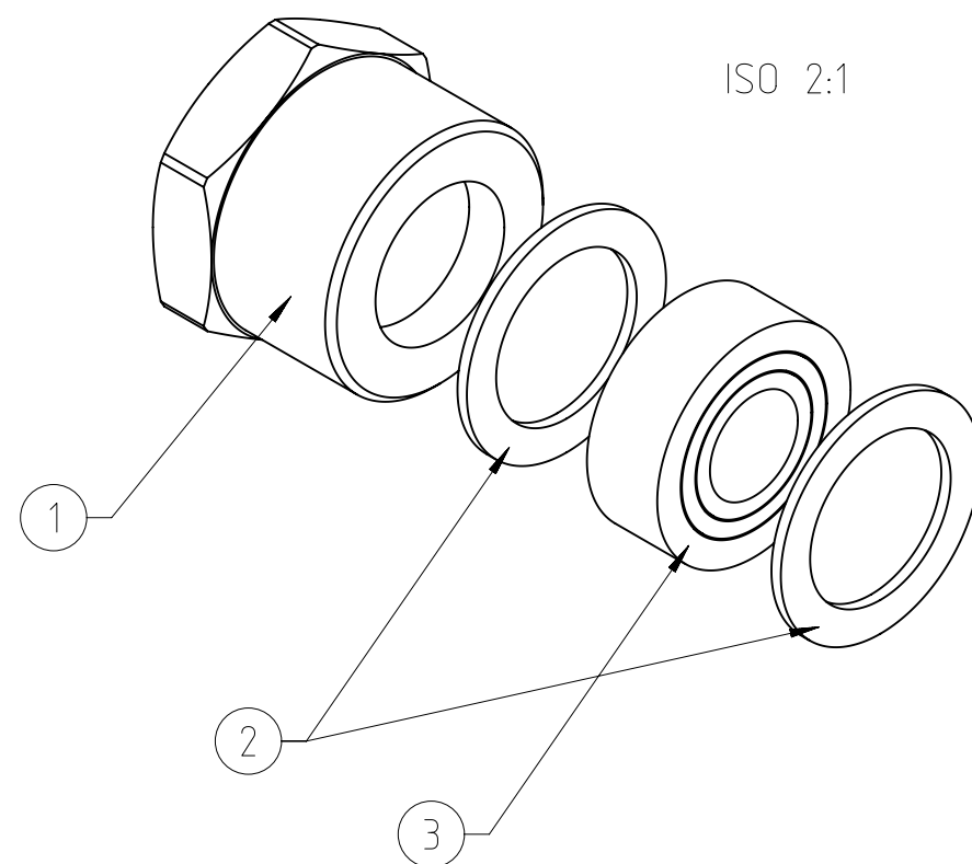
3 - Dichtring, ausschneidbar sealing with variable diameter
