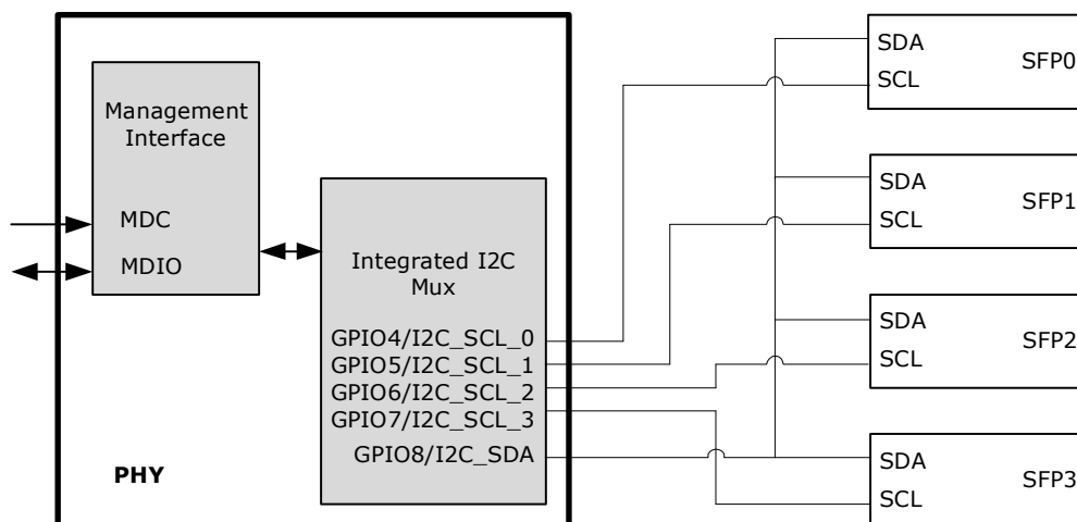
FIGURE 1-27: TWO-WIRE SERIAL MUX WITH SFP CONTROL AND STATUS
