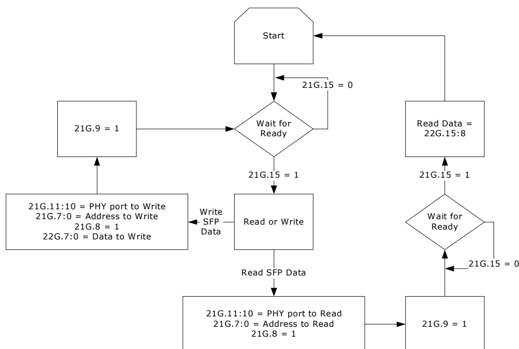
FIGURE 1-28: TWO-WIRE SERIAL MUX READ AND WRITE REGISTER FLOW
