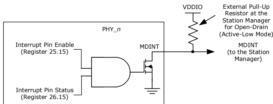
FIGURE 1-25: MDINT CONFIGURED AS AN OPEN-DRAIN (ACTIVE-LOW) PIN
