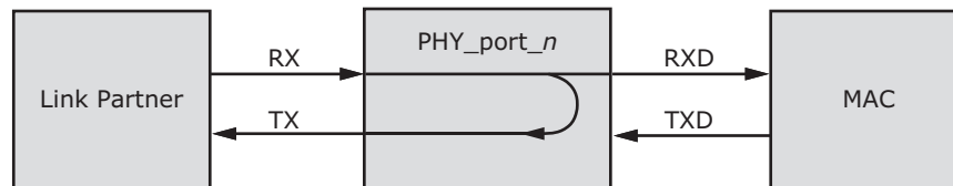
FIGURE 1-29: FAR-END LOOPBACK DIAGRAM
