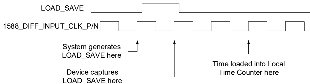
FIGURE 1-22: LOCAL TIME COUNTER LOAD/SAVE TIMING
