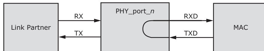
FIGURE 1-30: NEAR-END LOOPBACK DIAGRAM
