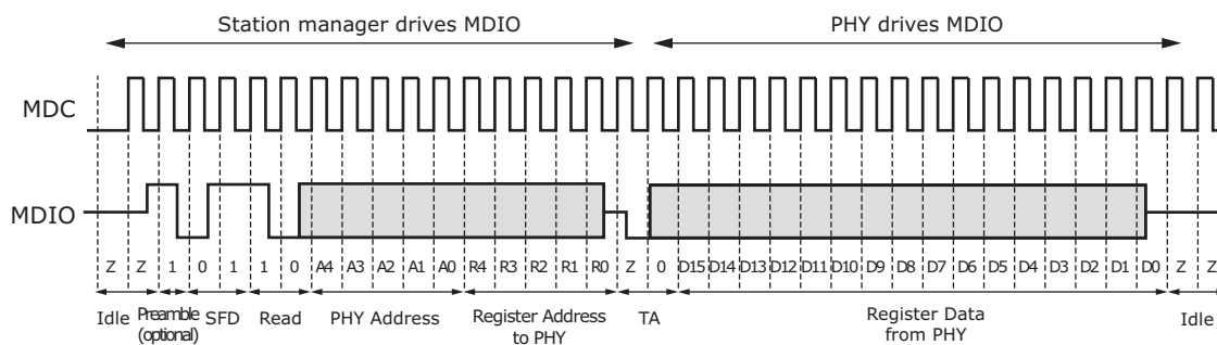
FIGURE 1-23: SMI READ FRAME
