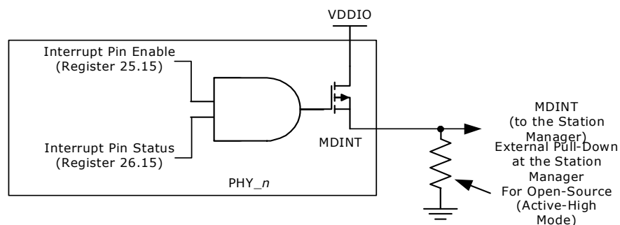
FIGURE 1-26: MDINT CONFIGURED AS AN OPEN-SOURCE (ACTIVE-HIGH) PIN
