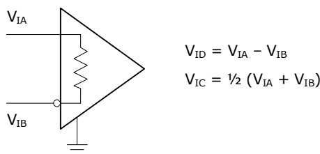
FIGURE 3-4: SGMII DC INPUT DEFINITIONS
