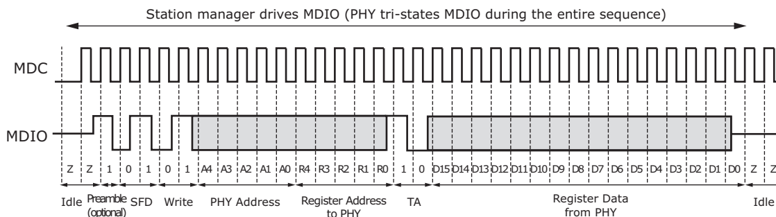
FIGURE 1-24: SMI WRITE FRAME
