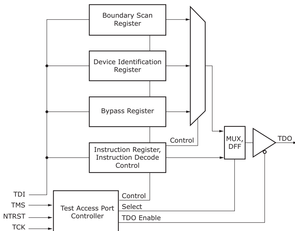
FIGURE 1-33: TEST ACCESS PORT AND BOUNDARY SCAN ARCHITECTURE
