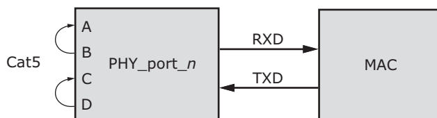
FIGURE 1-31: CONNECTOR LOOPBACK DIAGRAM
