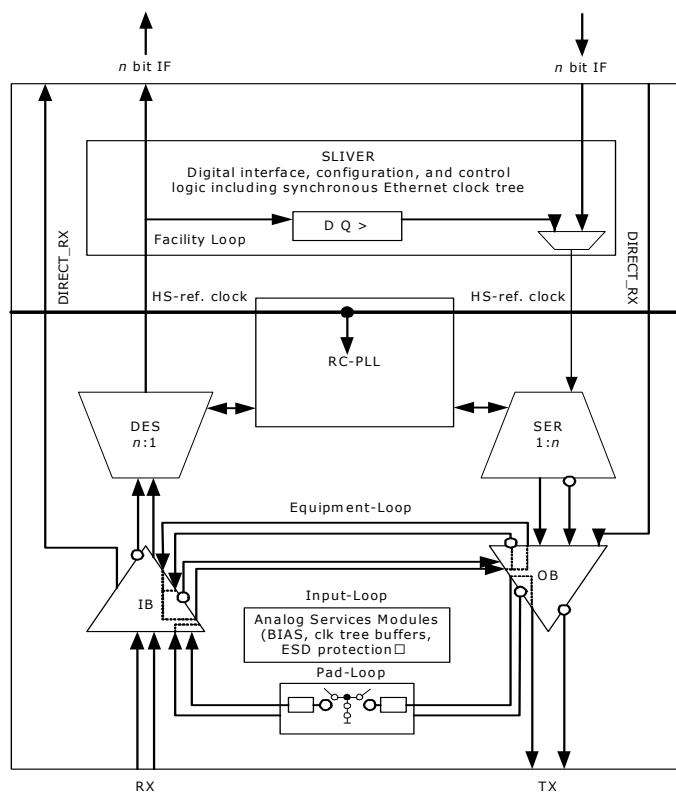
FIGURE 1-32: DATA LOOPS OF THE SERDES MACRO
