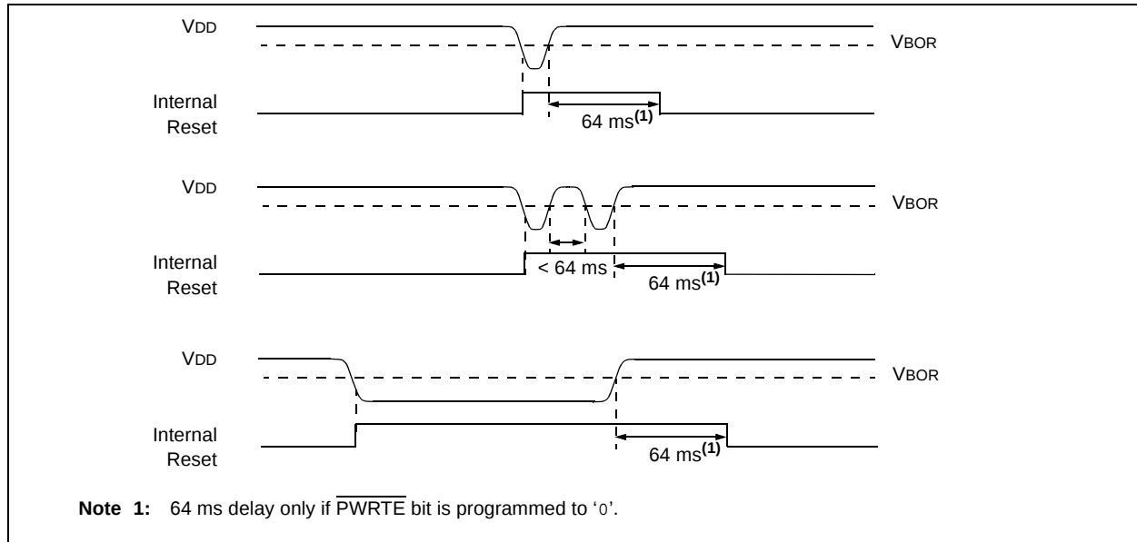
FIGURE 12-3: BROWN-OUT SITUATIONS
