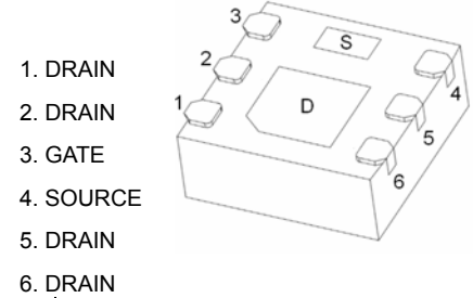
DFNWB2×2-6L
