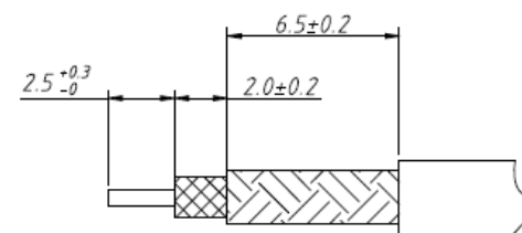
Wire stripping diagram
