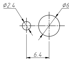
Mounting
