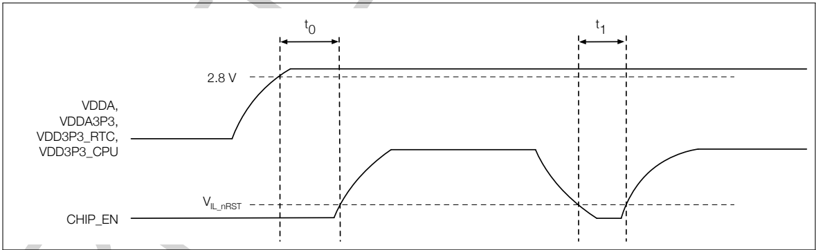
Figure 5: ESP8684 Series Power-up and Reset Timing
