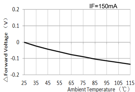
Ambient Temperature VS. \Delta Forward Voltage 环境温度与正向电压变化特性曲线
