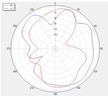
Theta=90 freq=1602MHz
