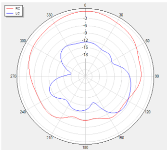
Phi=0 freq=1561MHz
