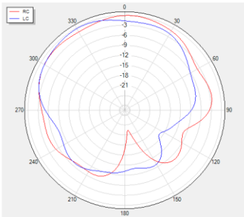
Phi=0 freq=1602MHz
