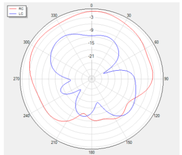
Phi=0 freq=1575MHz
