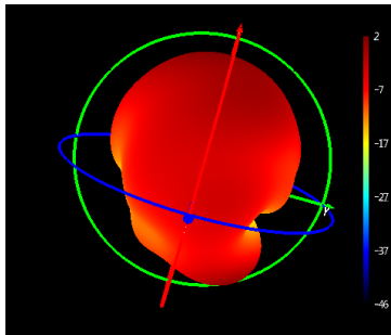
Phi=90 freq=1561MHz
