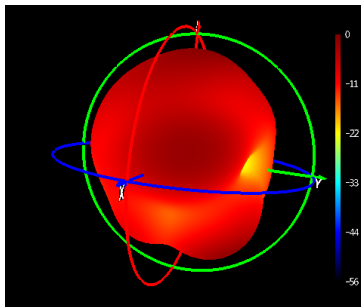
Phi=90 freq=1602MHz
