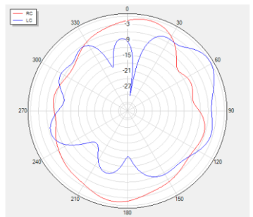
Theta=90 freq=1575MHz
