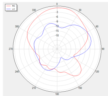
Phi=90 freq=1575MHz
