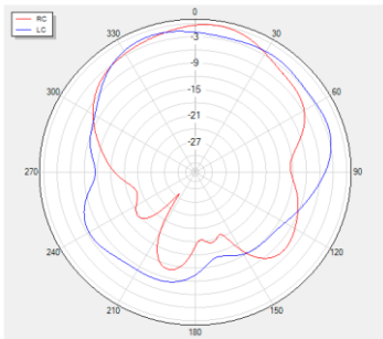
Phi=90 freq=1602MHz
