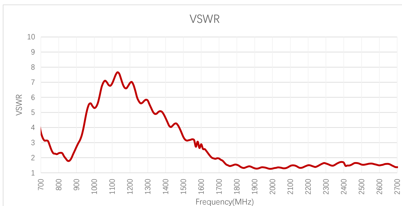
VSWR – 4G
