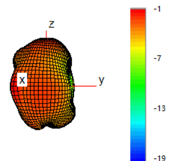
435 MHz
