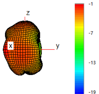
433 MHz
