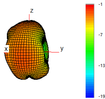
427 MHz
