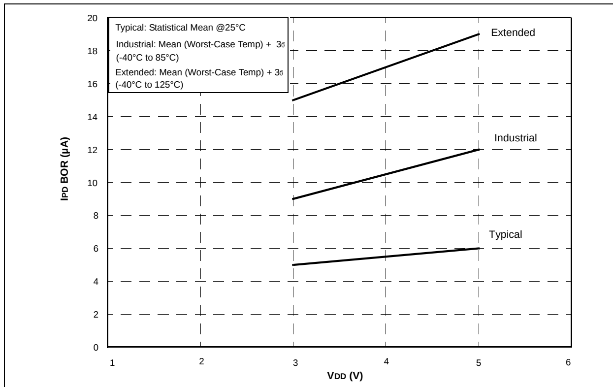
FIGURE 16-14: PIC16F610/616 I PD BOR vs. V DD
