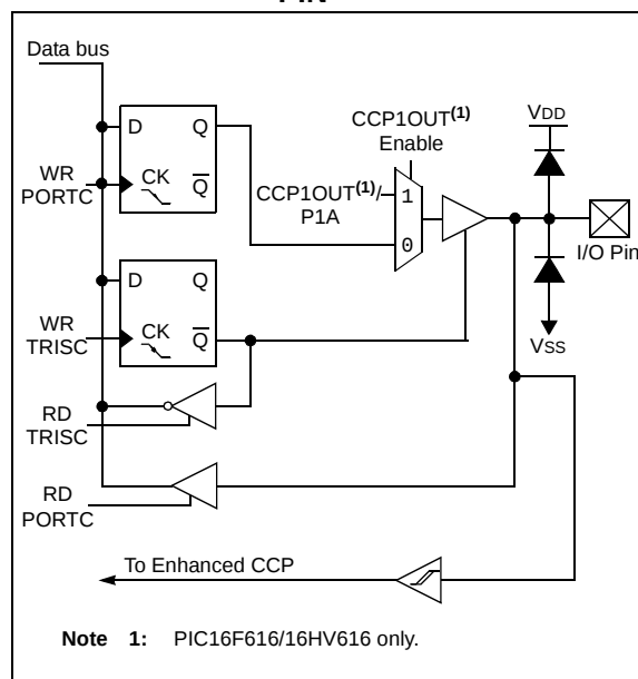
FIGURE 4-9: BLOCK DIAGRAM OF RC5 PIN
