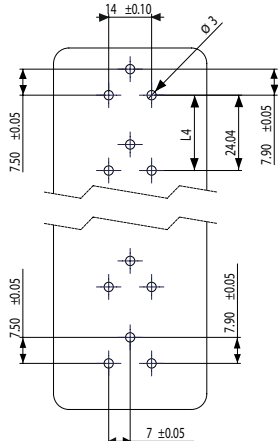
Drilling diagram for PCB terminals: L/N/PE individual [mm]
