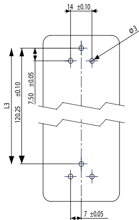
Drilling diagram for PCB terminals: L/N individual and PE bussed [mm]
