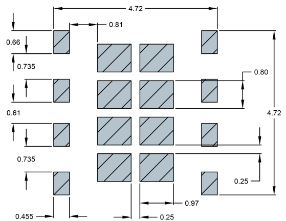
Recommended Solder Stencil
