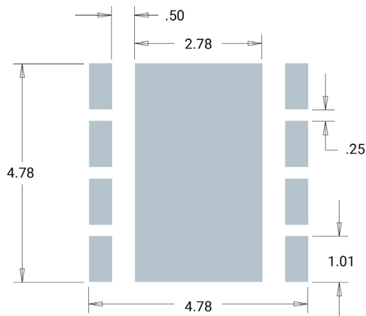
Recommended PCB Footprint
