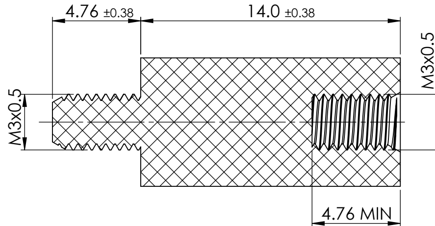
SECTION X-X
