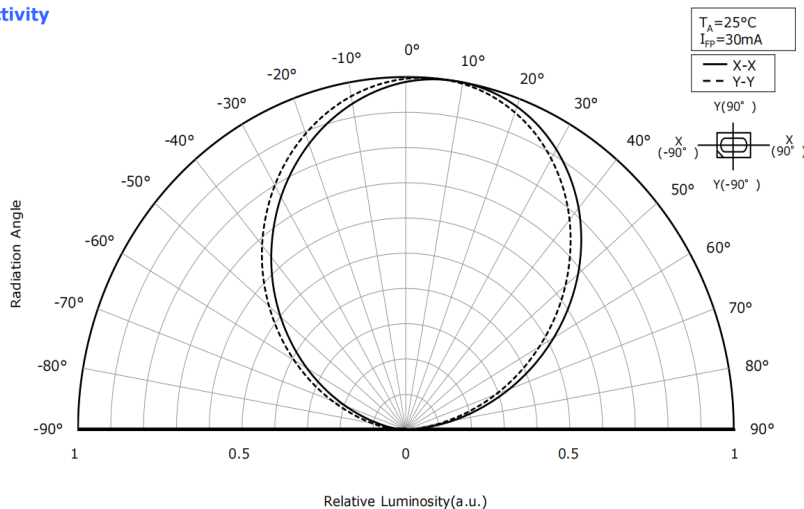
Directivity
