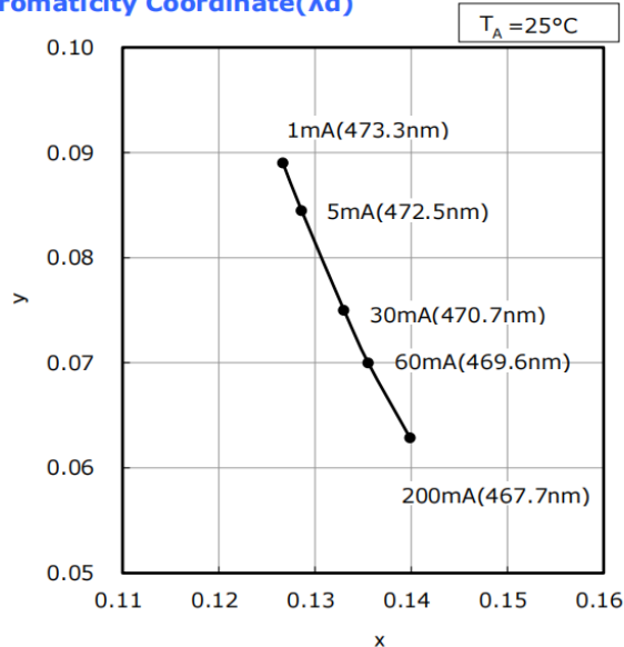
Forward Current vs Chromaticity Coordinate( \lambda_d )
