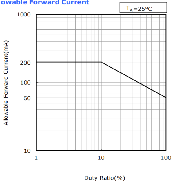
Duty Ratio vs Allowable Forward Current
