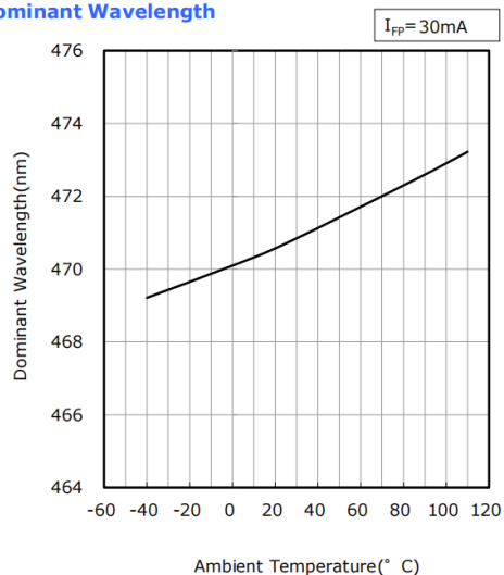
Ambient Temperature vs Dominant Wavelength
