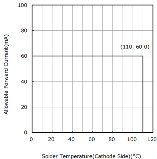
Solder Temperature(Cathode Side) vs Allowable Forward Current
