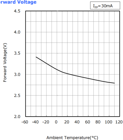
Ambient Temperature vs Forward Voltage
