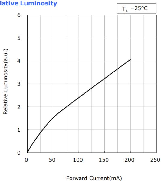
Forward Current vs Relative Luminosity
