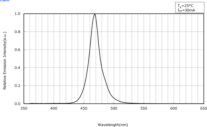
Spectrum
