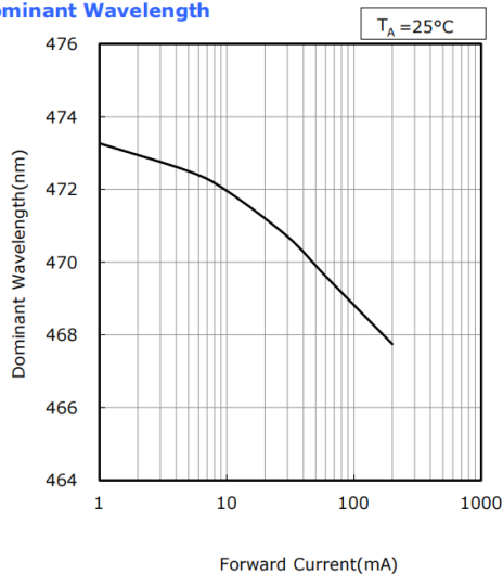
Forward Current vs Dominant Wavelength
