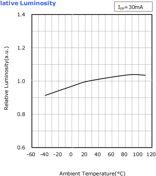
Ambient Temperature vs Relative Luminosity
