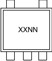
5-Lead SC-70
