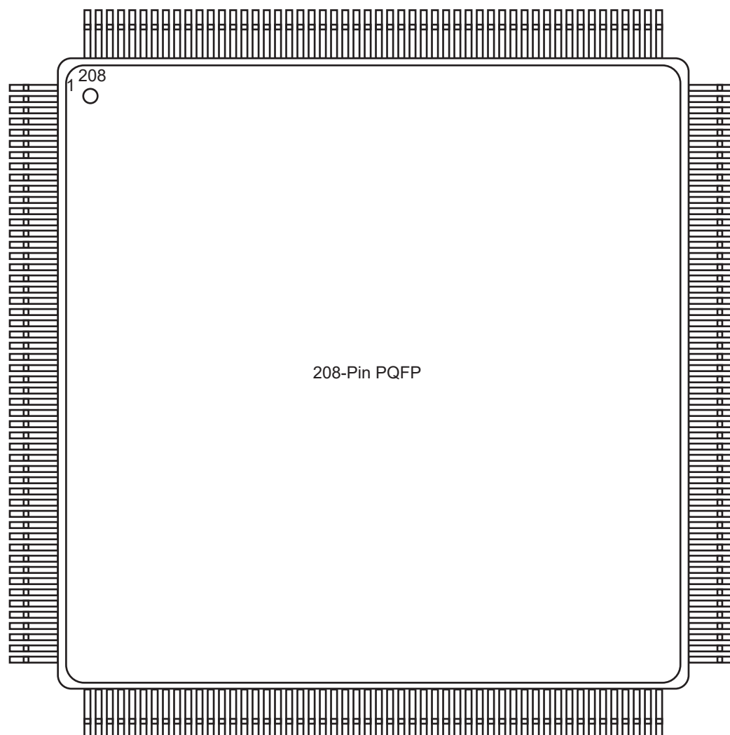
FIGURE 4-6 • PQ208—TOPVIEW
