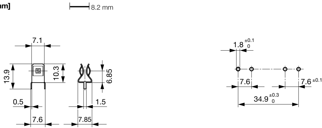
Drilling diagram
